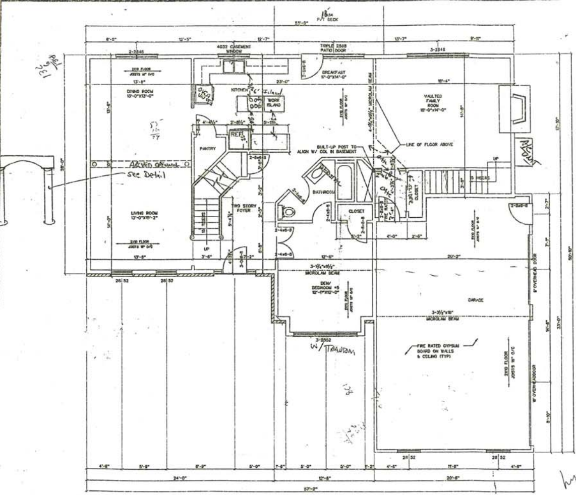
1 FIRST FLOOR PLAN SCALE: 1/8" = 1'-0"
