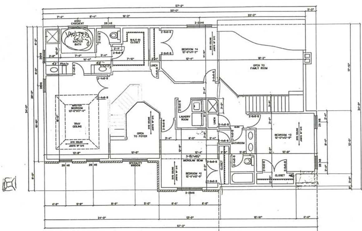
2 SECOND FLOOR PLAN SCALE: 1/8" = 1'-0"
